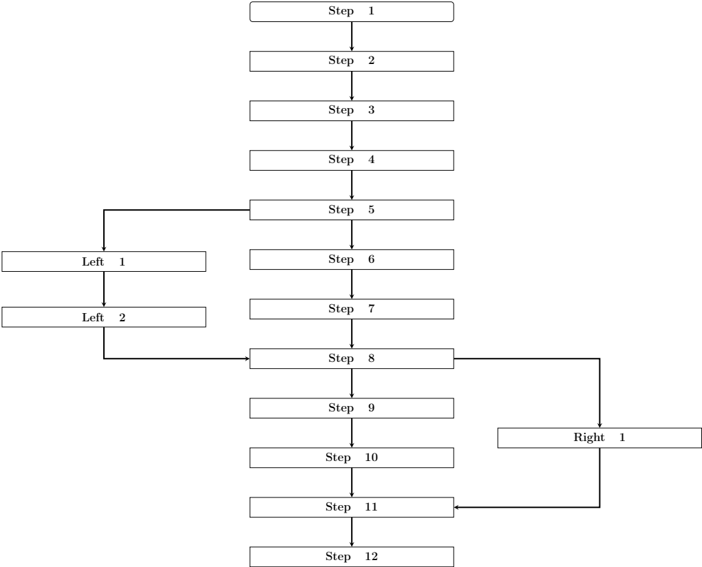
FIGURE 3.1: Study methodology.
