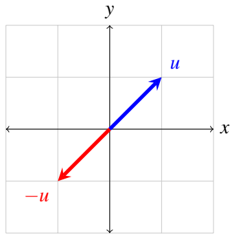
Figure 1: Vectors.
