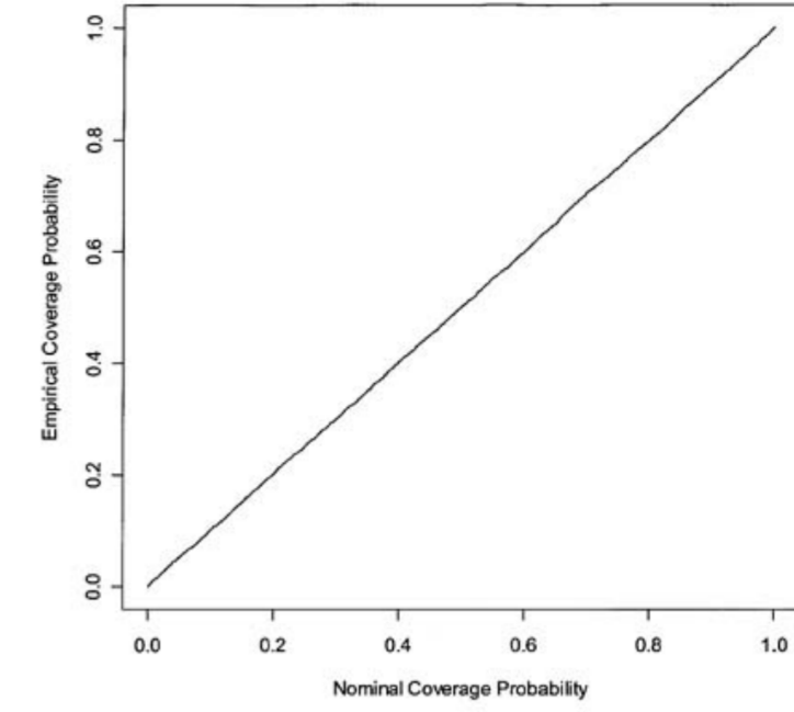
Figure 1: Empirical coverage of CIs for the relative-risk parameter \beta of haplotype 0100. Results are based on 10,000 simulated data sets with the same haplotype frequencies as the EUSSEN data. Haplotype 0100 has a multiplicative effect on disease risk, with \beta = 0.5 .
