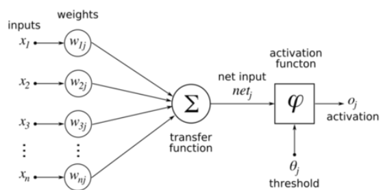
Figure 3.1: Rosenblatt's perceptron.
